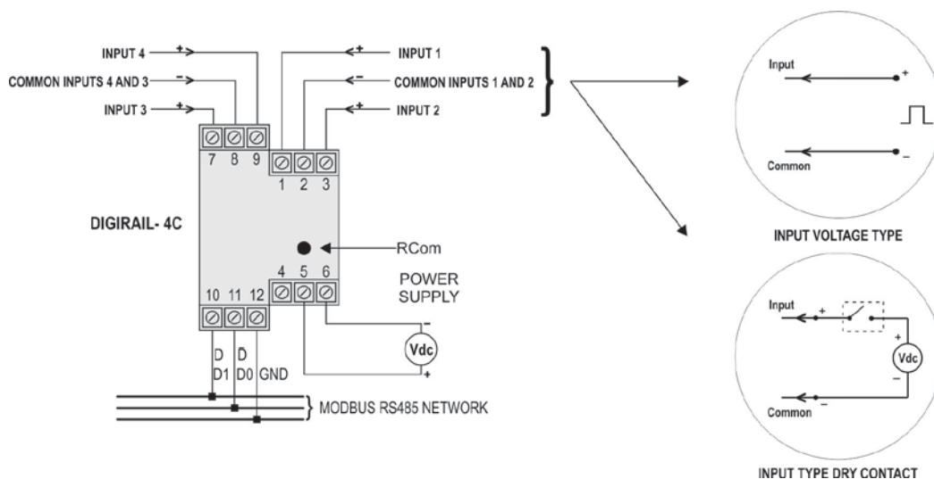
Figure 2 – Electrical Connections
